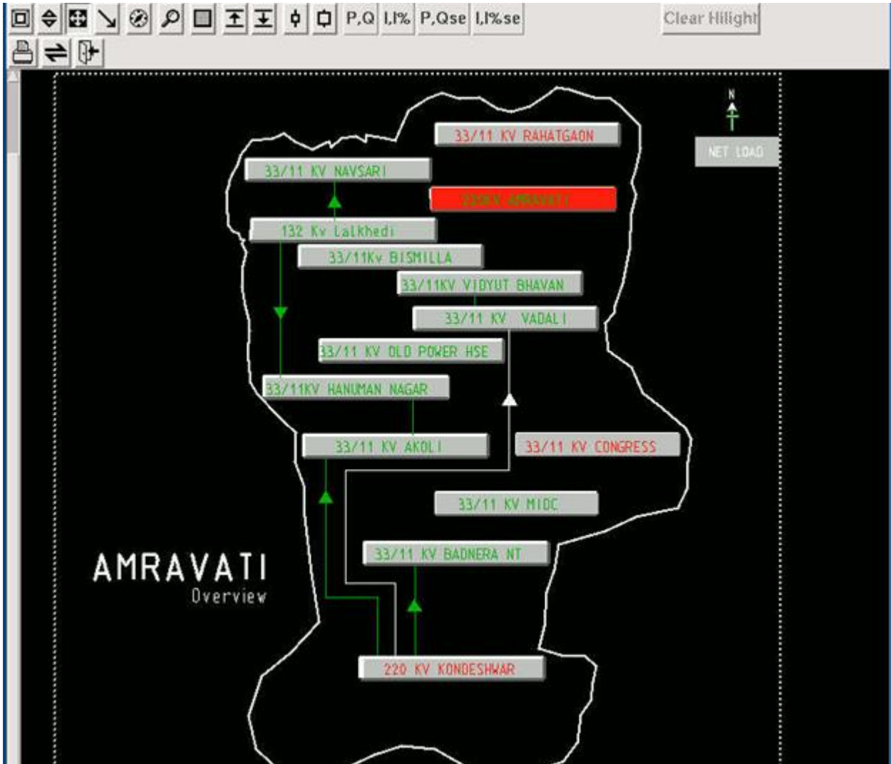
AMRAVATI TOWN OVERVIEW: Trip /shut down ON 220KV Amravati, thus it is shown blinking in red colour.
